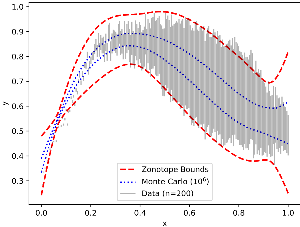
Chebyshev Basis ( p=3 )
